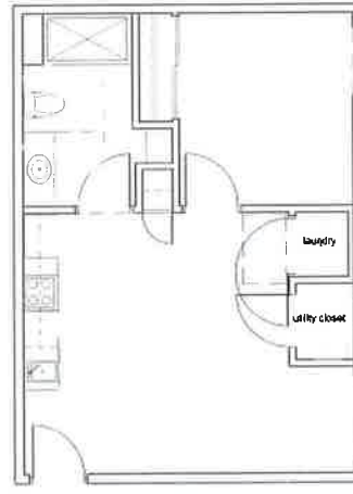
Unit B -1 Type A* 508 Sq. Ft
