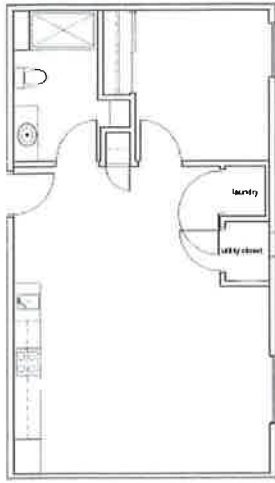
Unit A -1 Type B * 648 Sq. Ft
